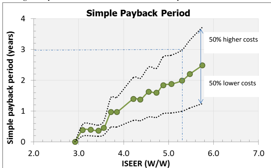
Fig. 7: Payback Period versus increased efficiency for room ACs in India 68
