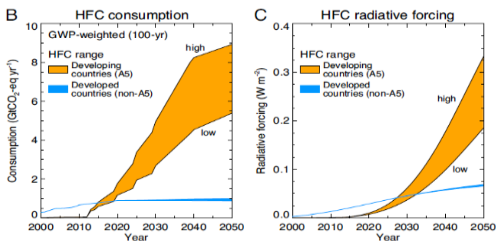
Fig. 1: Projected growth in HFCs and climate forcing from emissions
