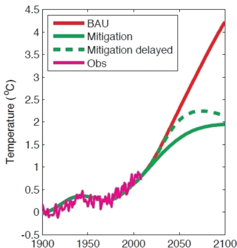
Figure 5: Temperature Consequences of Delayed SLCP Mitigation
