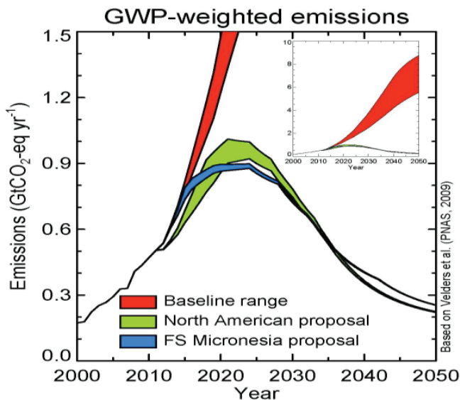
Figure 10: Projected HFC Emission Reductions from FSM and NA Proposals
