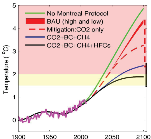
Figure 4: Warming Avoided Through Combined SLCP and CO 2 Mitigation
