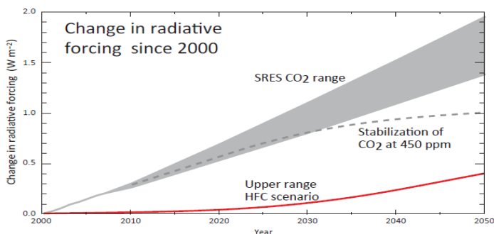
Figure 1: By 2050 forcing from HFCs could equal 20-40% of the growth of CO 2 forcing since 2000
