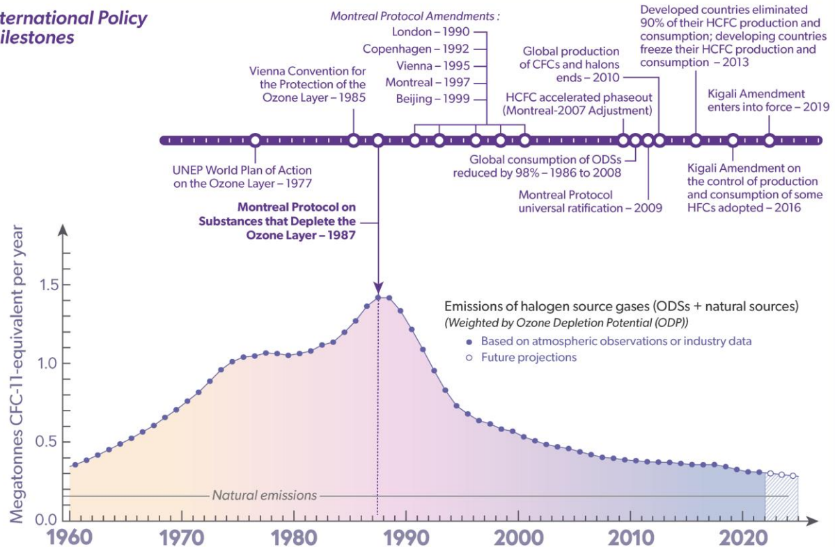
Figure 6. Stratospheric Ozone Depletion and Policy Milestones
